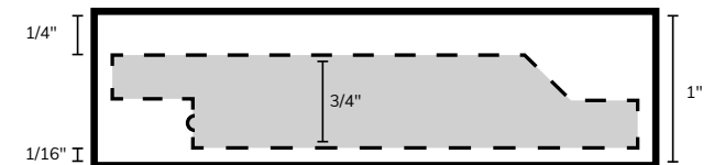
DISCOLORATION: ROUGH BOARD, AFTER SURFACING 1/8 INCH AND AFTER SURFACING 1/4 INCH FROM ROUGH
